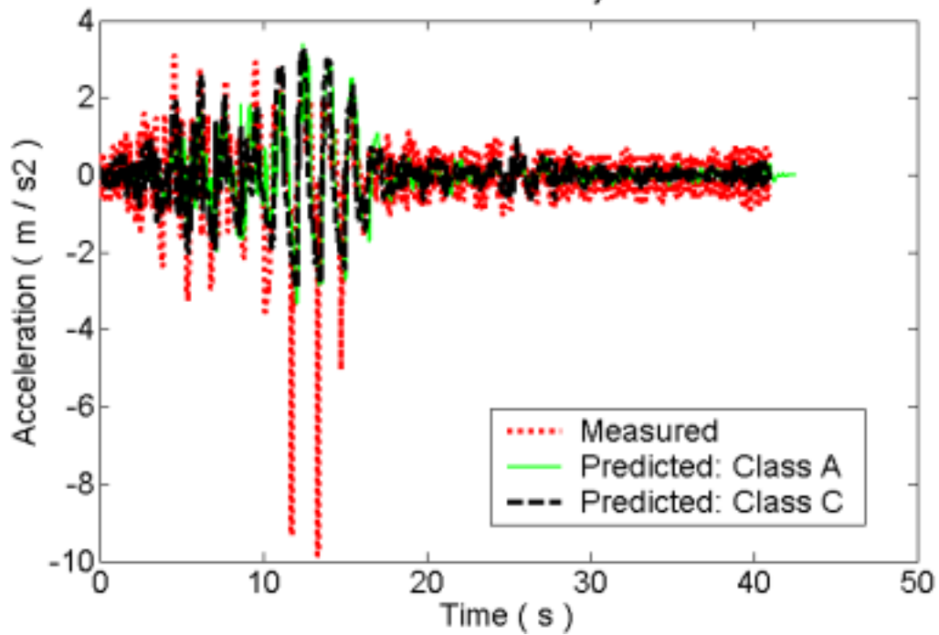
Acceleration time history at ACC04
