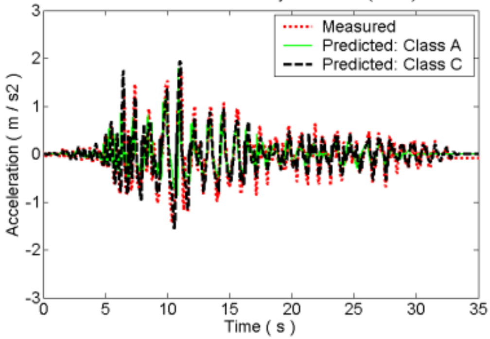
Acceleration time history at ACC07 (A475)
