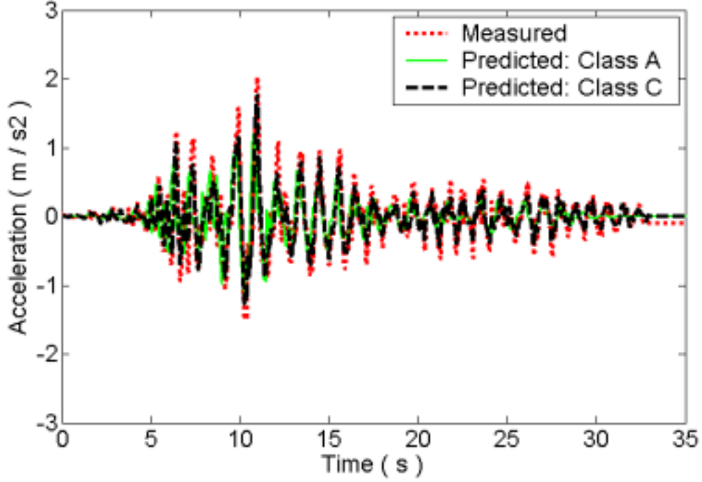
Acceleration time history at ACC01 (A475)
