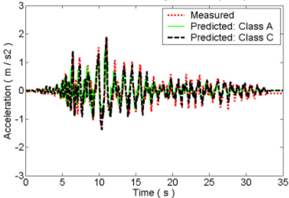
Acceleration time history at ACC05 (A475)
