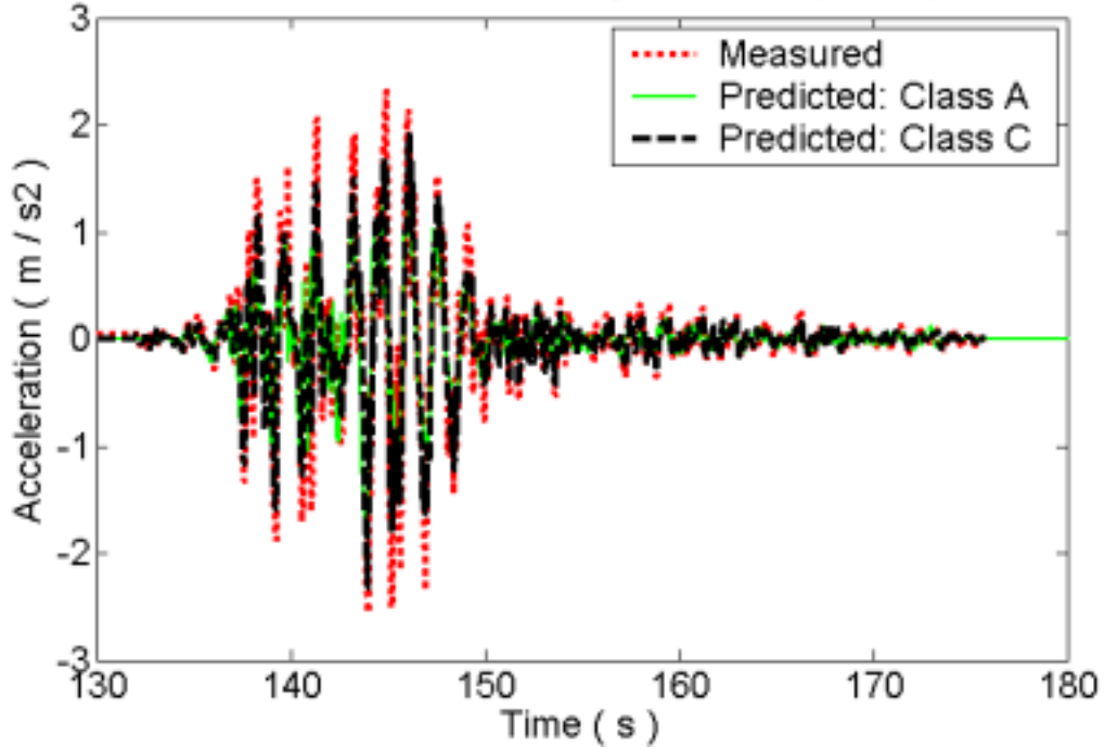
Acceleration time history at ACC01 (A2475)
