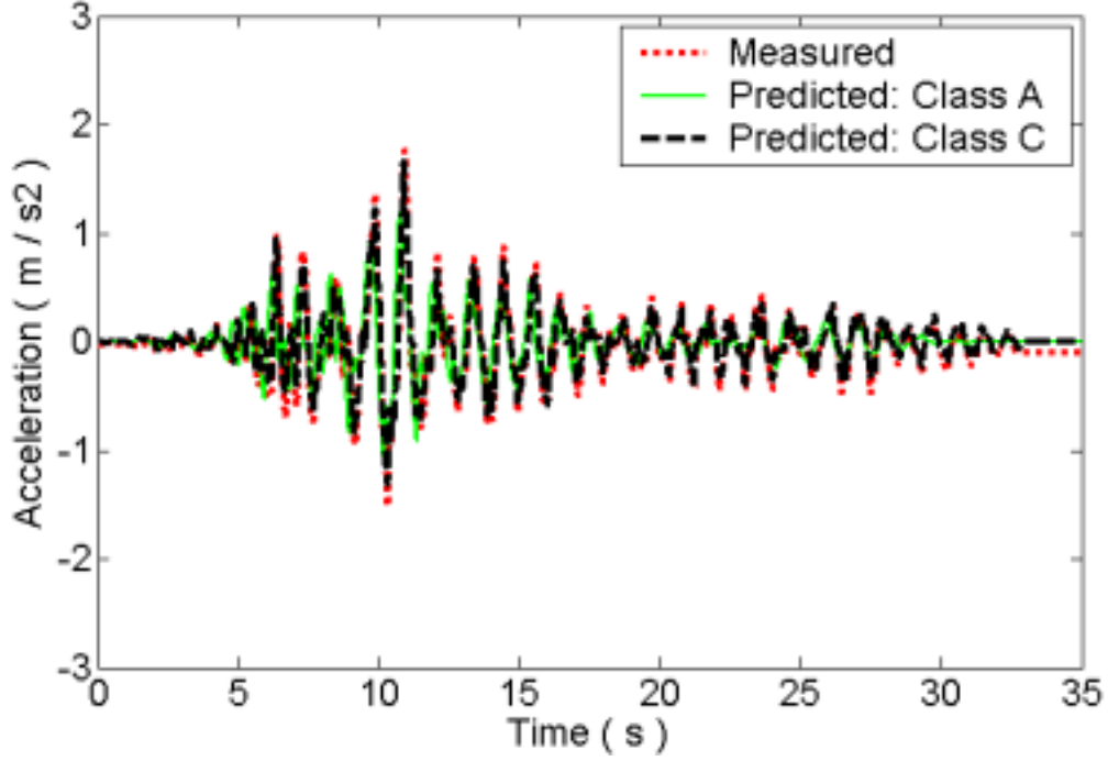
Acceleration time history at ACC04 (A475)
