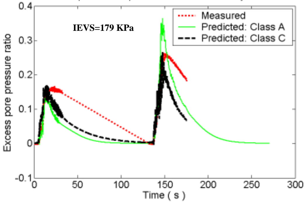
Excess pore water pressure ratio time history at EPP4
