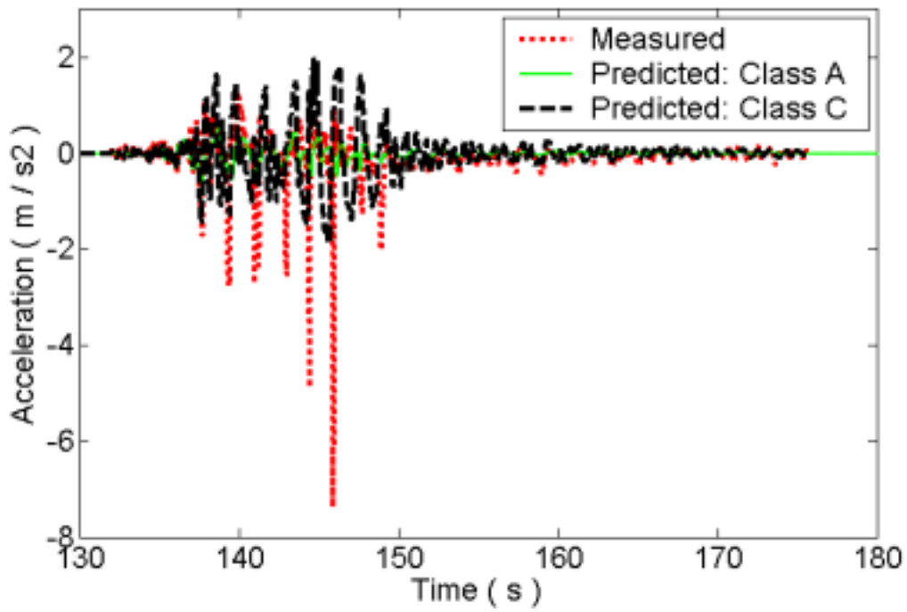
Acceleration time history at ACC03 (A2475)
