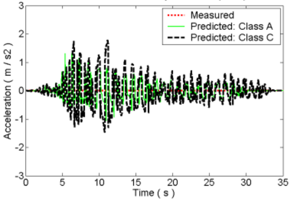
Acceleration time history at ACC09 (A475)
