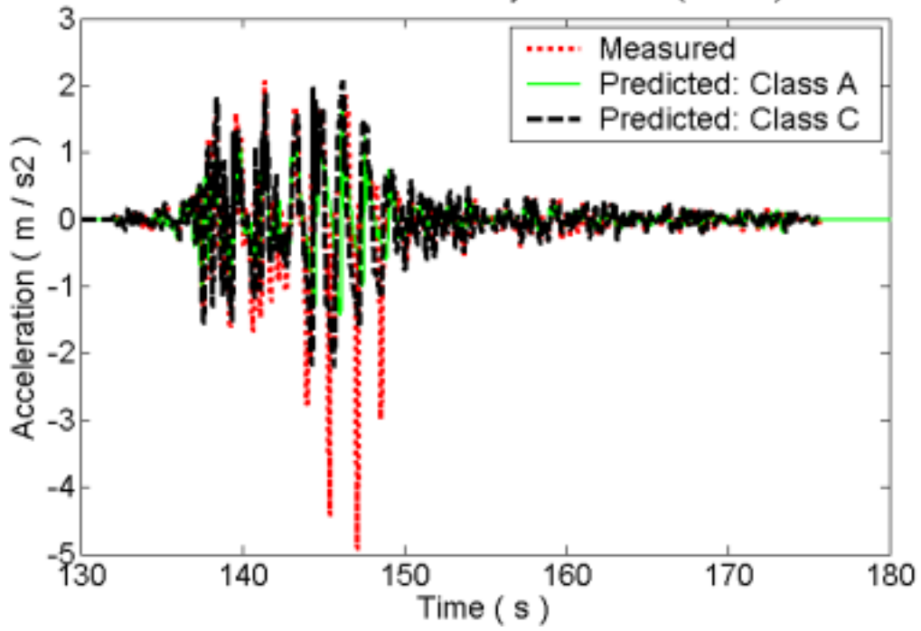
Acceleration time history at ACC06 (A2475)
