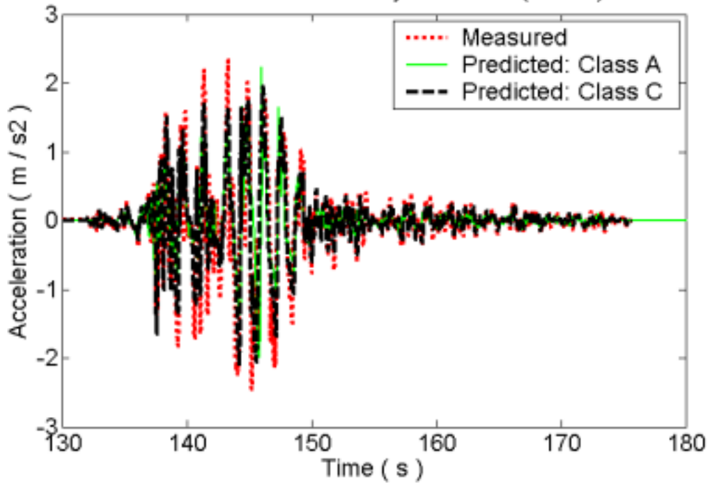
Acceleration time history at ACC07 (A2475)
