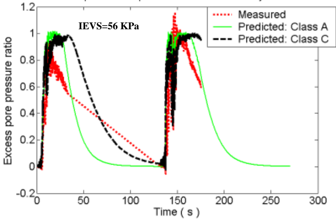
Excess pore water pressure ratio time history at EPP2
