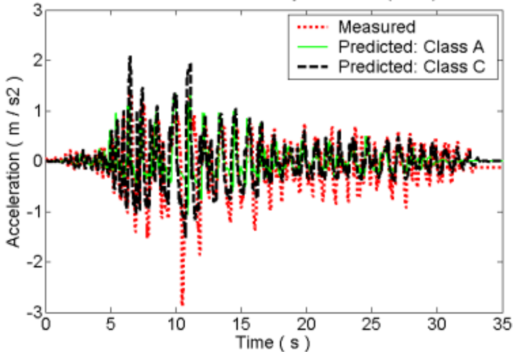
Acceleration time history at ACC08 (A475)
