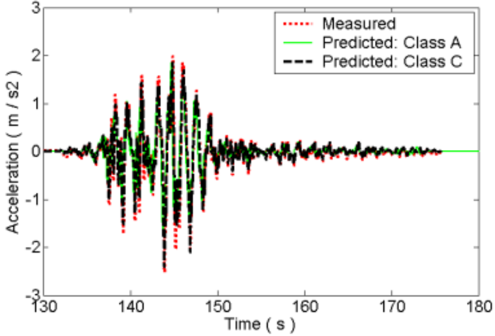
Acceleration time history at ACC04 (A2475)
