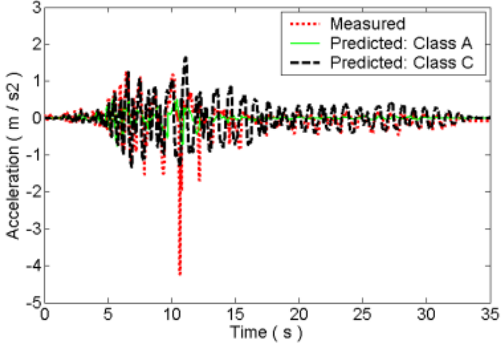
Acceleration time history at ACC03 (A475)
