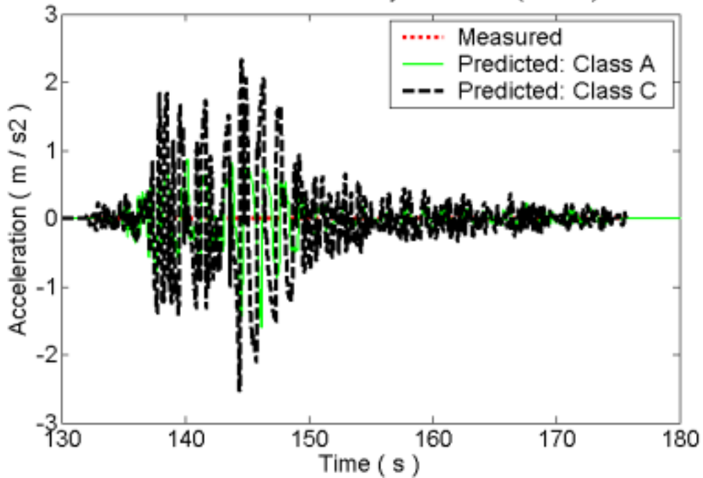
Acceleration time history at ACC09 (A2475)
