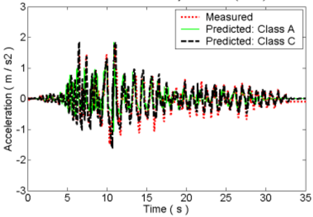
Acceleration time history at ACC06 (A475)
