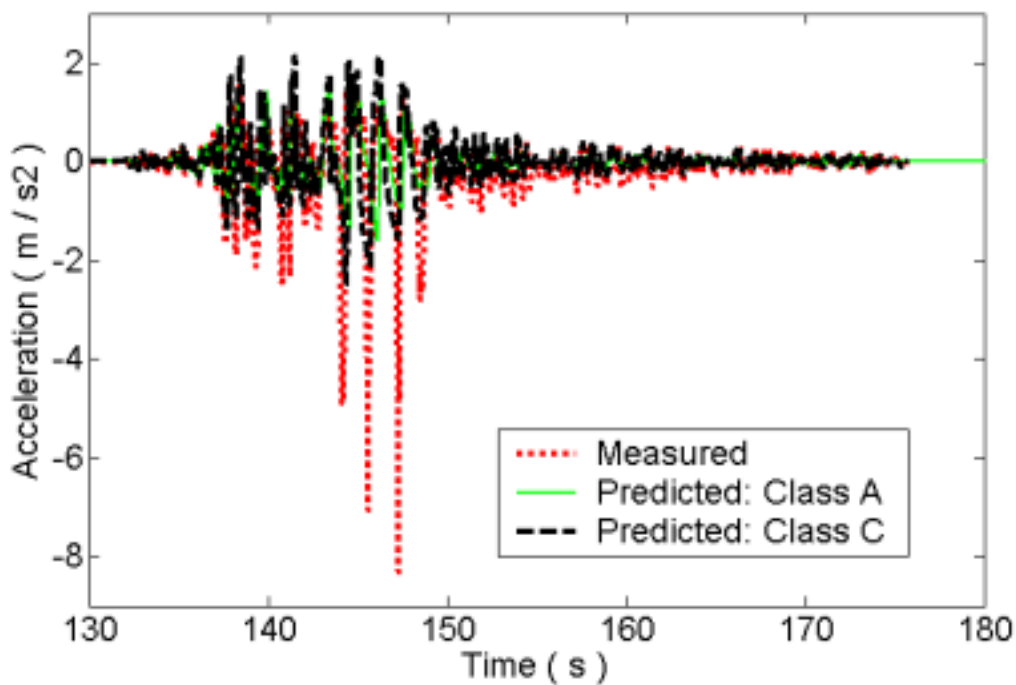
Acceleration time history at ACC08 (A2475)
