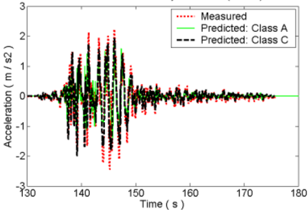
Acceleration time history at ACC05 (A2475)
